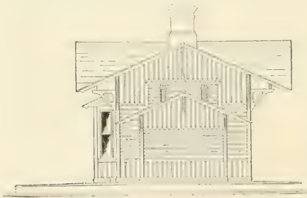
FIG. 513.—END ELEVATION.
