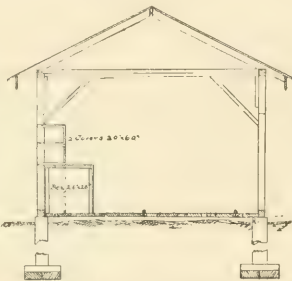
FIG. 26.—CROSS-SECTION.
