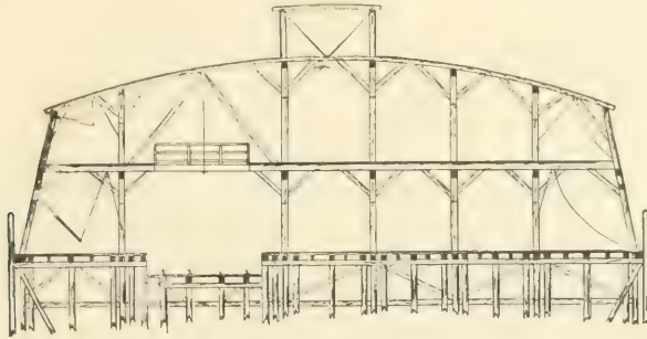
FIG. 393. CROSS-SECTION.
