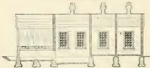
FIG. 207.—LONGITUDINAL SECTION.
