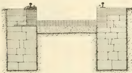
FIG. 148.—CROSS-SECTION.
