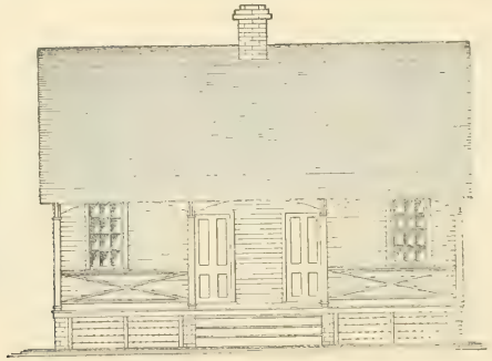
FIG. 62.—FRONT ELEVATION.
