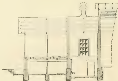
FIG. 202.—LONGITUDINAL SECTION.
