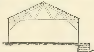
FIG. 189.—CROSS-SECTION.
