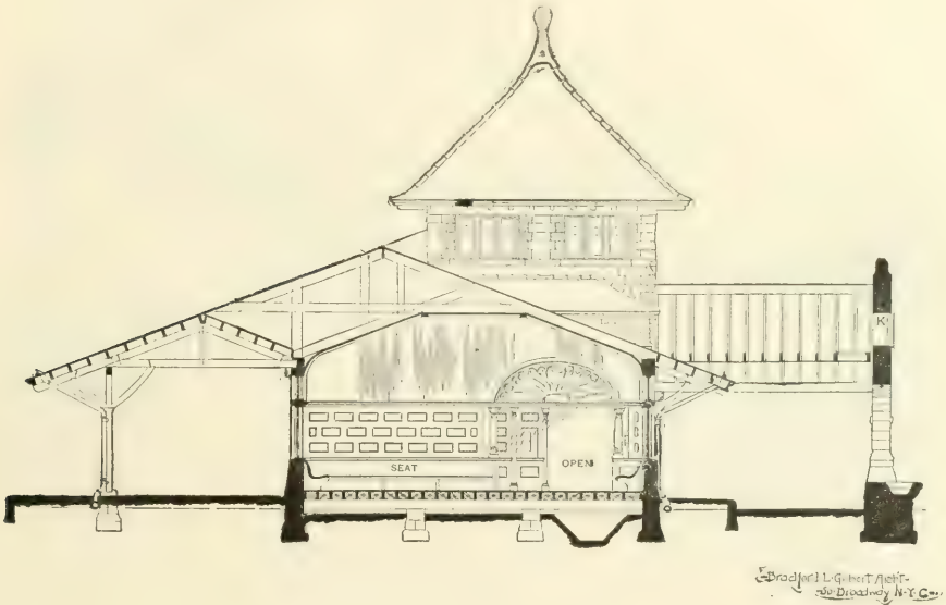
FIG. 579.—CROSS-SECTION.
