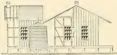
FIG. 69.—END ELEVATION AND CROSS SECTION.
