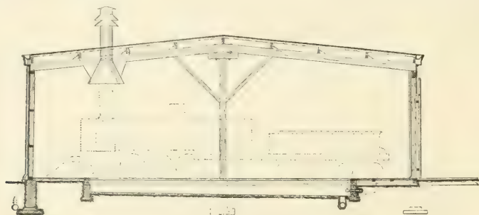
FIG. 331.—CROSS-SECTION.
