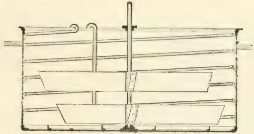
FIG. 221.—CROSS-SECTION OF TANK.
