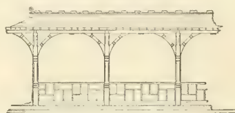
FIG. 404.—FRONT ELEVATION.
