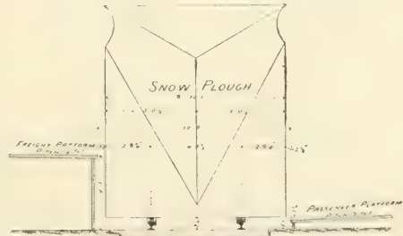
FIG. 401.—CROSS-SECTION.
