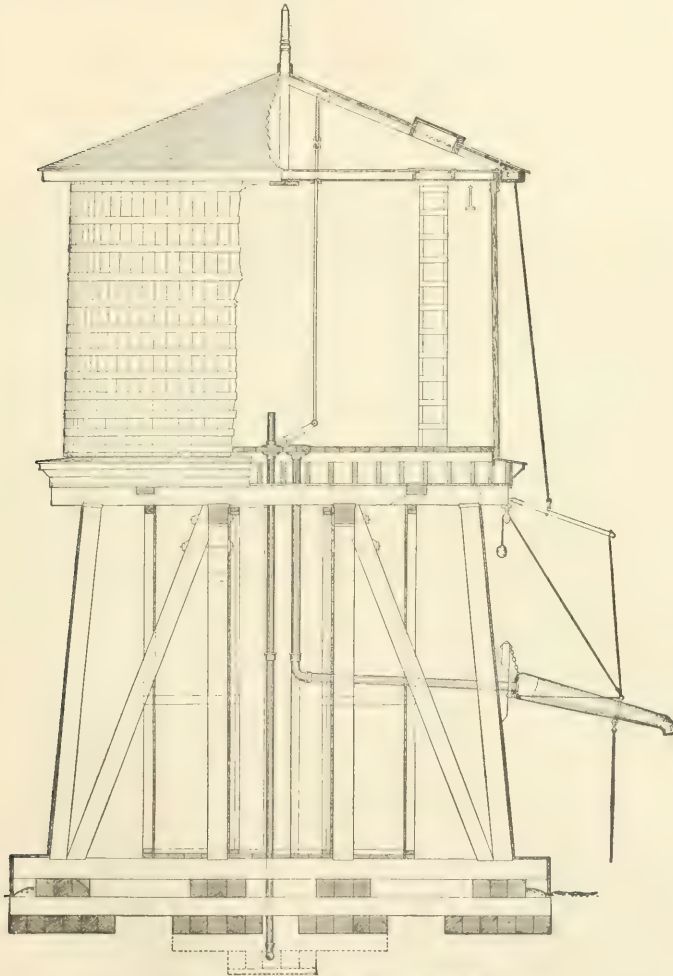
FIG. 262.—ELEVATION AND CROSS-SECTION.
