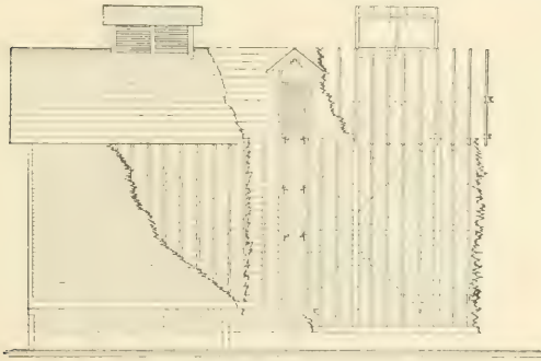
FIG. 165.—FRONT ELEVATION.
