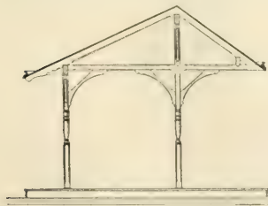
FIG. 402.—CROSS-SECTION.
