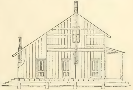
FIG. 58.—CROSS-SECTION.
