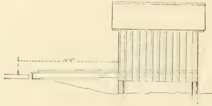
FIG. 37. SIDE ELEVATION.
