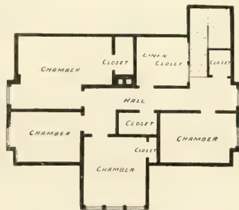
FIG. 501.—SECOND-FLOOR PLAN.
