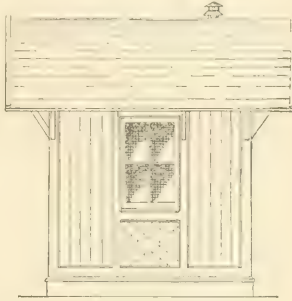
FIG. 15.—SIDE ELEVATION.
