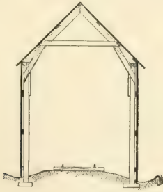
FIG. 103.—CROSS-SECTION.
