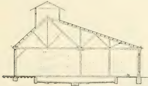
FIG. 322.—CROSS-SECTION.
