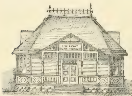
FIG. 93.—FRONT ELEVATION.
