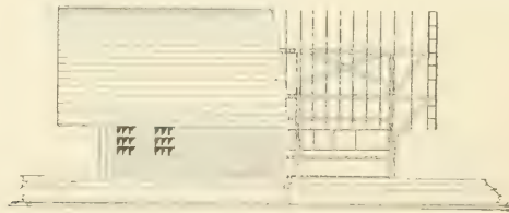
FIG. 361.—FRONT ELEVATION.
