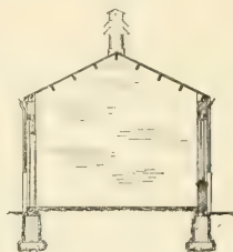
FIG. 206.—END ELEVATION.
