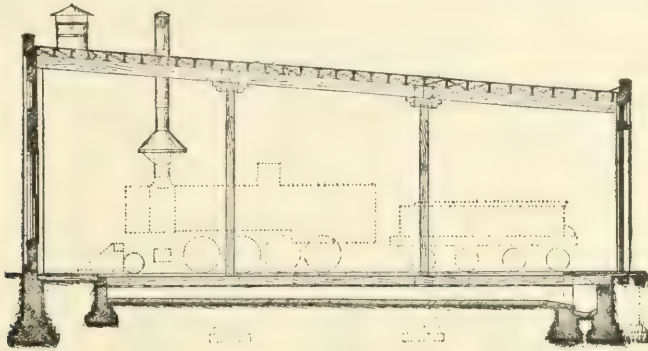
FIG. 333.—CROSS-SECTION.
