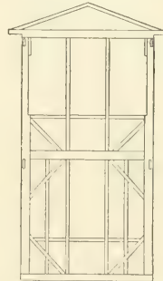
FIG. 122.—ELEVATION OF FRAME.
