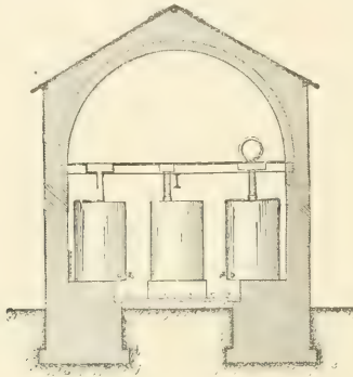
FIG. 190.—CROSS-SECTION.
