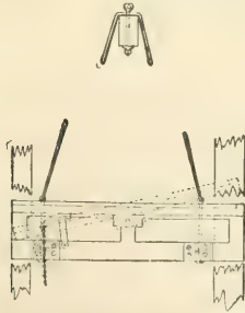
FIG. 167.—ELEVATION OF HOISTING-CAGE.
