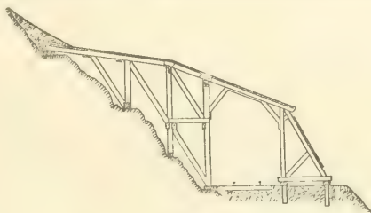
FIG. 108.—CROSS-SECTION.
