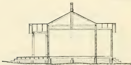
FIG. 503.—CROSS-SECTION.
