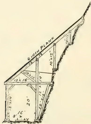
FIG. 112.—CROSS-SECTION.
