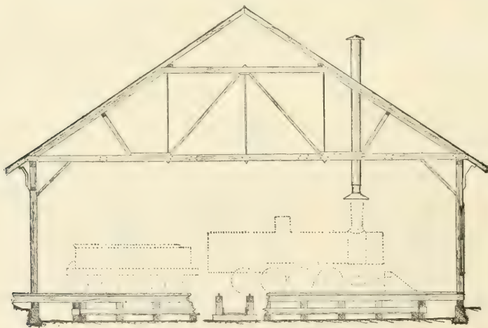
FIG. 321.—CROSS-SECTION.
