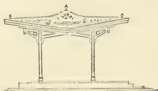
FIG. 406.—END ELEVATION.
