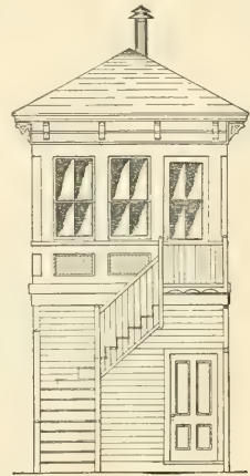
FIG. 124.—SIDE ELEVATION.
