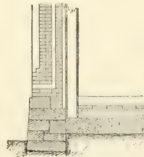
FIG. 173.—DETAIL SECTION OF WALL AND FLOOR.
