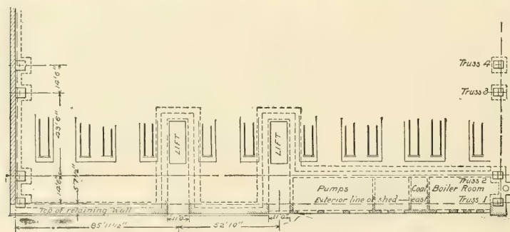
FIG. 665.—PLAN OF FOUNDATIONS.
