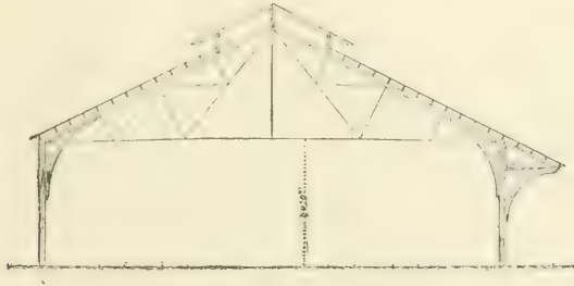
FIG. 629.—CROSS SECTION OF TRAIN SHED.
