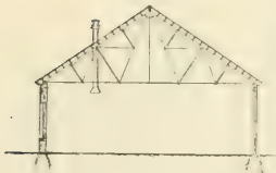
FIG. 342.—CROSS-SECTION.
