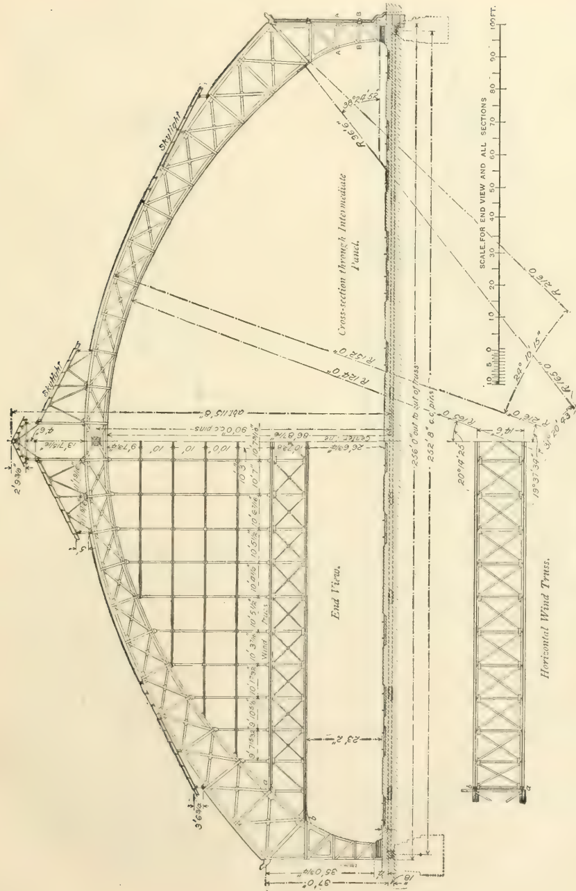
FIG. 658.—SECTION AND END ELEVATION OF TRAIN-SHED.
