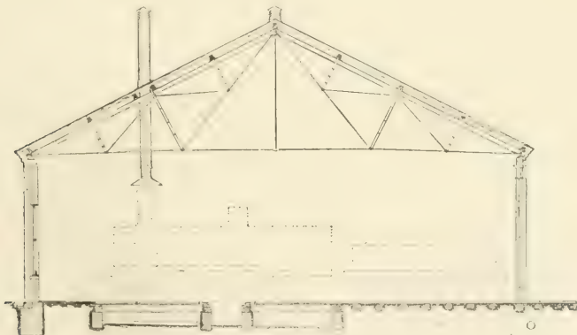
FIG. 315.—CROSS-SECTION.
