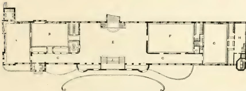
FIG. 648.—GROUND-PLAN OF MAIN FLOOR.
