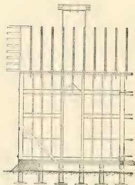
FIG. 169.—ELEVATION OF FRAME.
