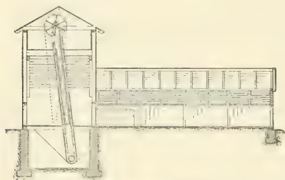
FIG. 181.—LONGITUDINAL SECTION.
