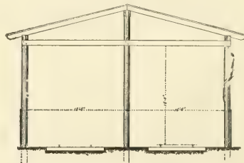
FIG. 133.—CROSS-SECTION.
