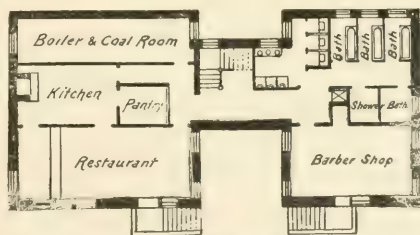
FIG. 97.—BASEMENT-FLOOR PLAN.
