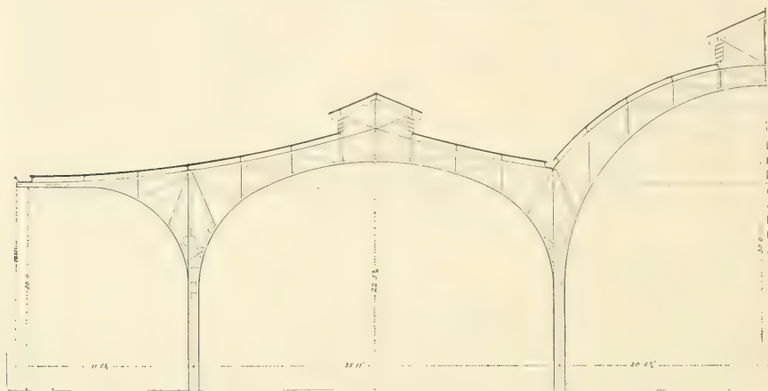
FIG. 669.—CROSS SECTION OF TRAIN-SHED.
