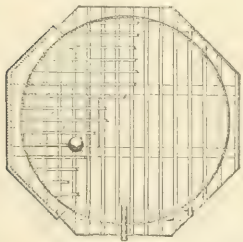
FIG. 252.—GROUND-PLAN OF FLOOR FRAMING.
