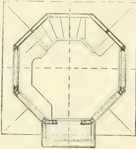
FIG. 117.—SECOND-FLOOR PLAN.
