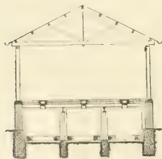
FIG. 203.—CROSS-SECTION.
