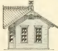
FIG. 432.—END ELEVATION.
