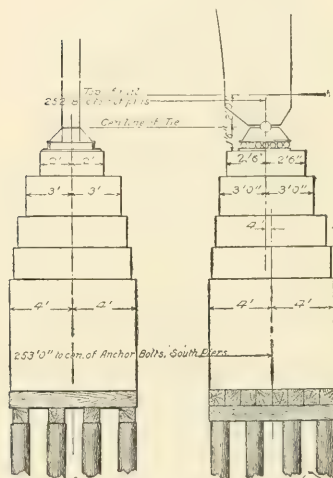
FIG. 663.—DETAILS OF MOVABLE END OF ARCH.
