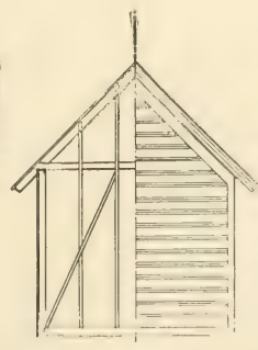
FIG. 34.—SIDE ELEVATION.
