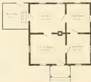
FIG. 73. — GROUND PLAN.
