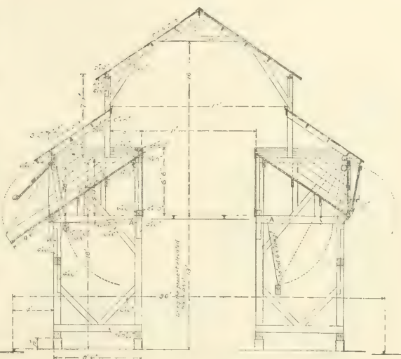
FIG. 292.—CROSS-SECTION.
