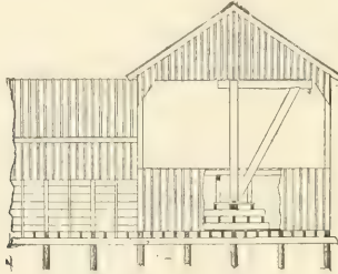
FIG. 267.—FRONT ELEVATION.
