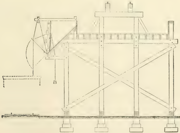
FIG. 278.—CROSS-SECTION.
