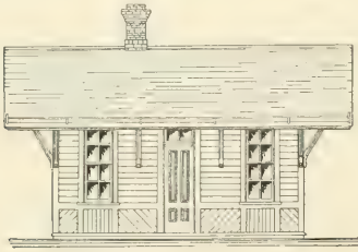
FIG. 476.—FRONT ELEVATION.
