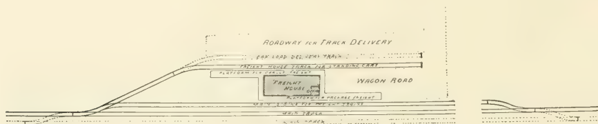
FIG. 354.—PROPOSED GENERAL LAYOUT FOR LOCAL FREIGHT-STATION.
