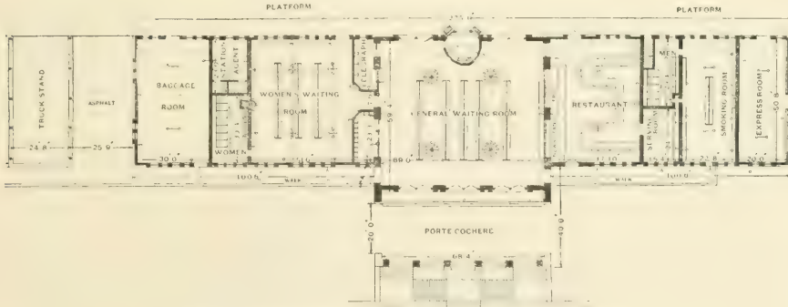
FIG. 623.—GROUND-PLAN OF MAIN FLOOR, LYMAN STREET BUILDING.
