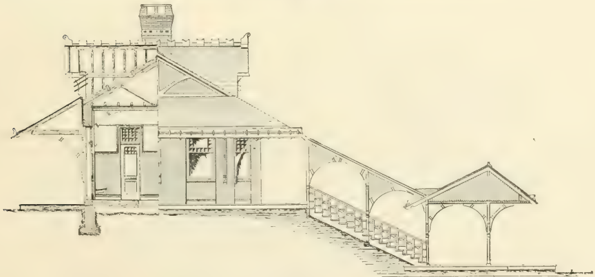
FIG. 552.—CROSS-SECTION AND END ELEVATION.
