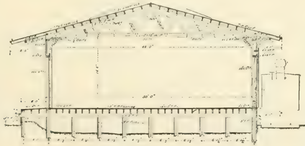
FIG. 377.—CROSS-SECTION.
