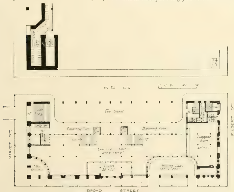
FIG. 690.—GROUND-PLAN OF FIRST FLOOR.
