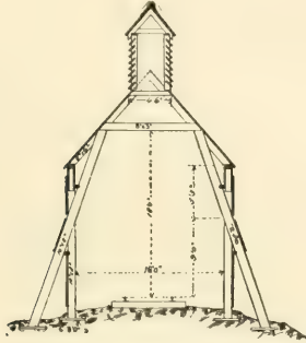
FIG. 100.—CROSS-SECTION.
