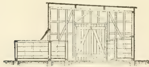
FIG. 174 — CROSS-SECTION.
