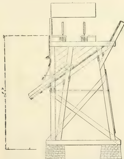
FIG. 299.—CROSS SECTION WITH HIGH-CHUTES.
