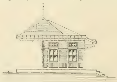
FIG. 485.—END ELEVATION.
