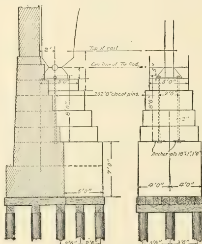
FIG. 664.—DETAILS OF FIXED END OF ARCH.
