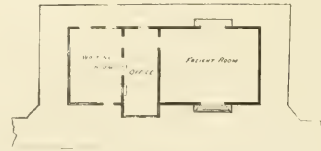
FIG. 428.—GROUND-PLAN, CLASS "E."
