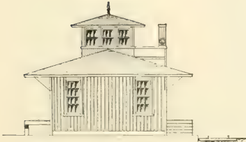
FIG. 119.—END ELEVATION.
