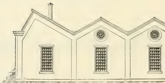
FIG. 348.—SIDE ELEVATION.
