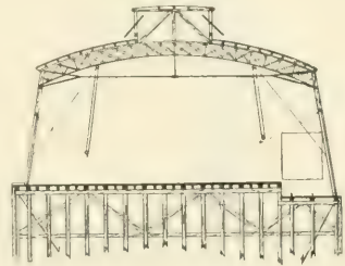
FIG. 387.—CROSS-SECTION.
