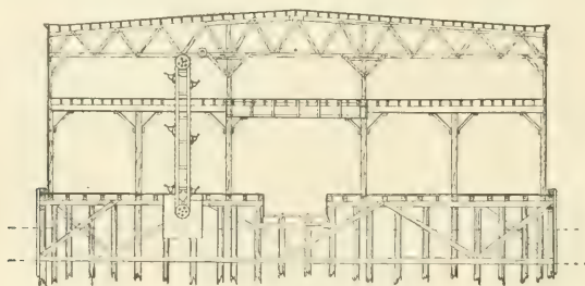
FIG. 395.—CROSS-SECTION.
