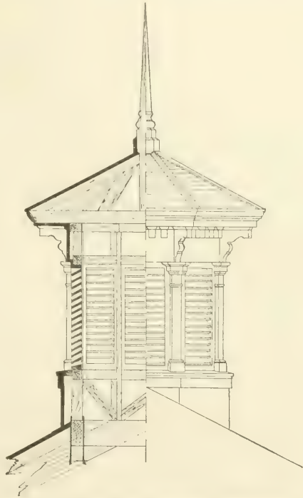
FIG. 313.—ELEVATION AND SECTION OF VENTILATOR.
