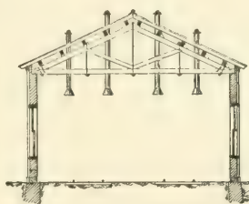
FIG. 129.—CROSS-SECTION.
