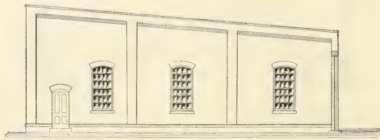
FIG. 337.—END ELEVATION.
