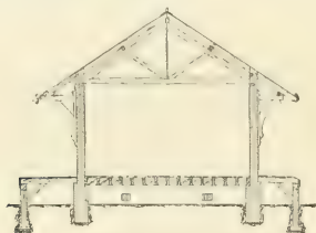
FIG. 368. CROSS-SECTION.
