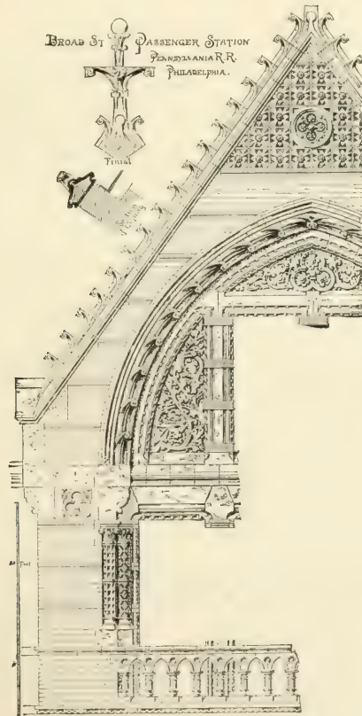
FIG. 641.—DETAIL OF EXTERIOR.
