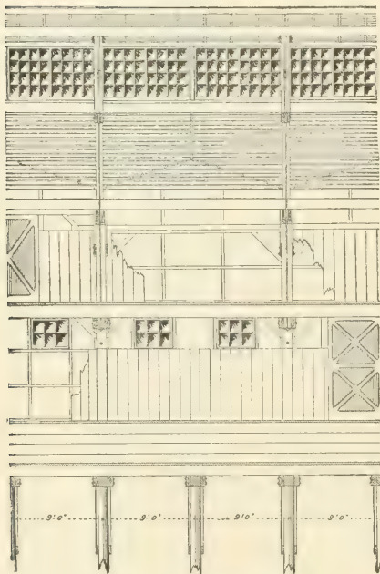
FIG. 391.—LONGITUDINAL SECTION.
