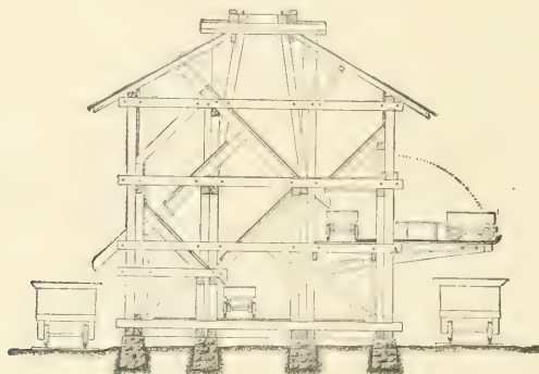
FIG. 280.—CROSS-SECTION.
