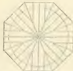
FIG. 253.—GROUND-PLAN OF ROOF FRAMING.
