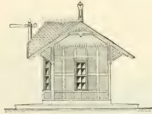
FIG. 481.—END ELEVATION.
