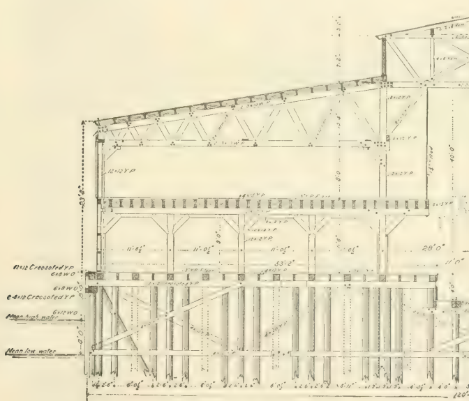
FIG. 390.—CROSS-SECTION.
