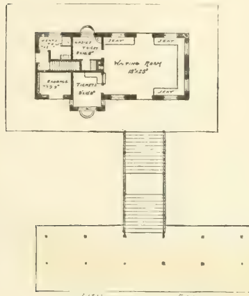
FIG. 602.—GROUND-PLAN, QUEEN'S LANE DEPOT.
