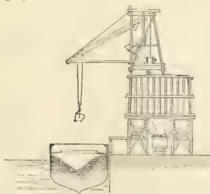
FIG. 303.—CROSS-SECTION.
