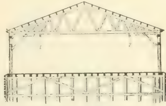
FIG. 397.—CROSS SECTION.
