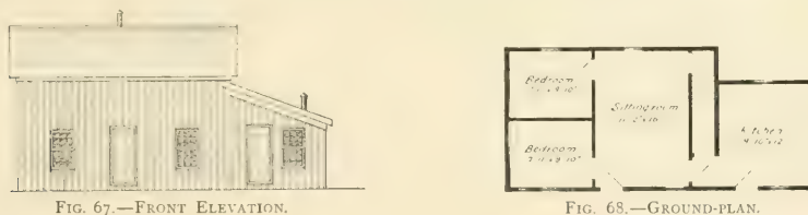
FIG. 67.—FRONT ELEVATION.
