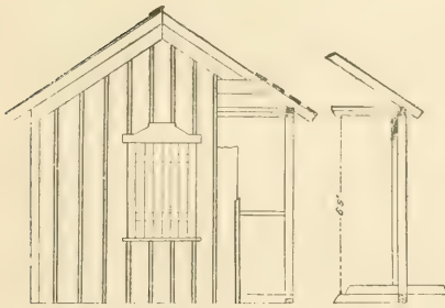
FIG. 23.—END ELEVATION AND CROSS-SECTION.
