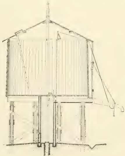
FIG. 261.—CROSS-SECTION.
