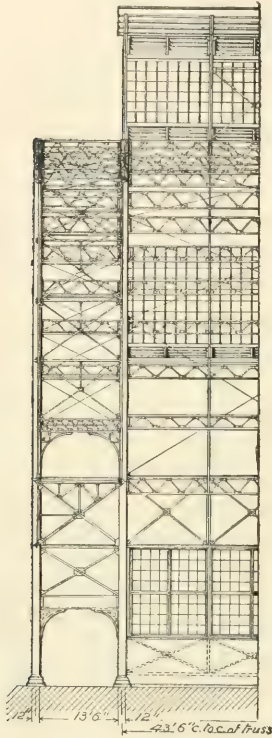
FIG. 659.—LONGITUDINAL SECTION OF TRAIN SHED.
