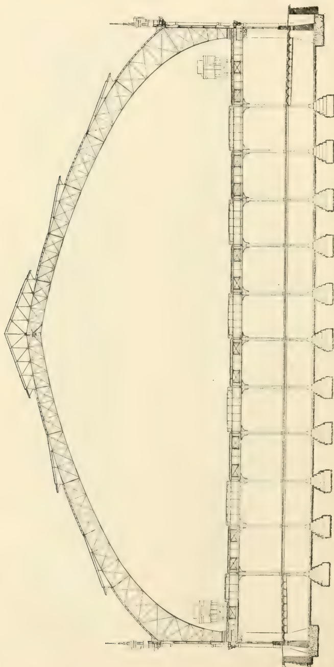
FIG. 688.—CROSS-SECTION OF TRAIN-SHED.
