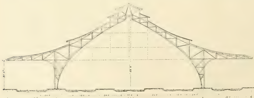
FIG. 670.—CROSS SECTION OF TRAIN-SHED.
