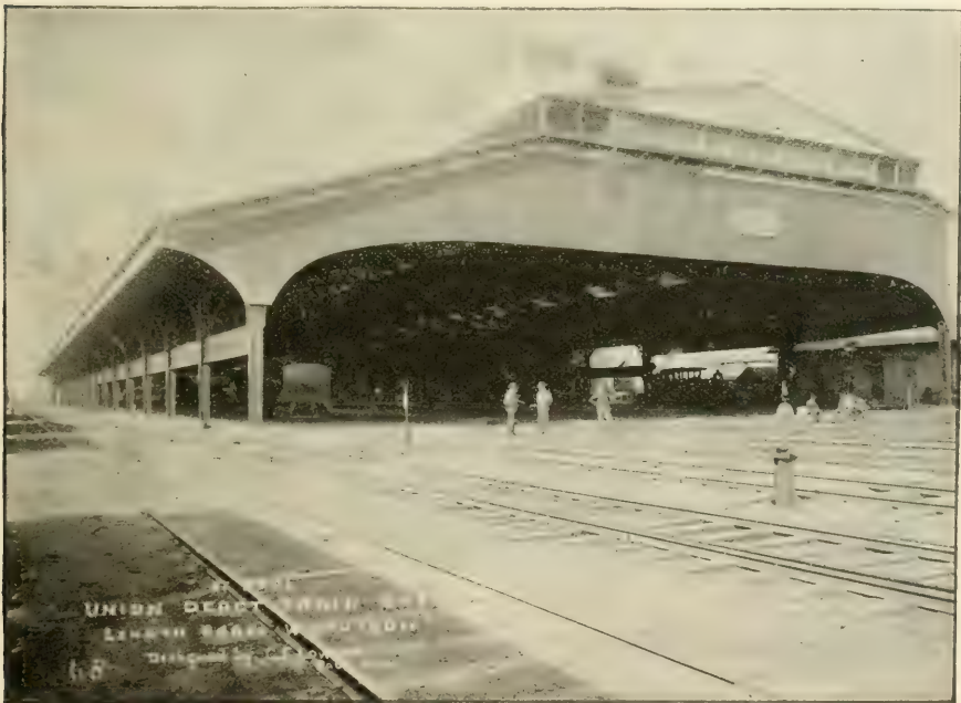
FIG. 676.—PERSPECTIVE OF EXTERIOR OF TRAIN-SHED.
