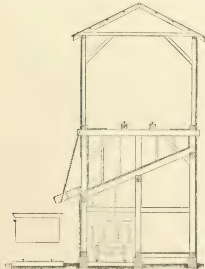
FIG. 283.—CROSS-SECTION.
