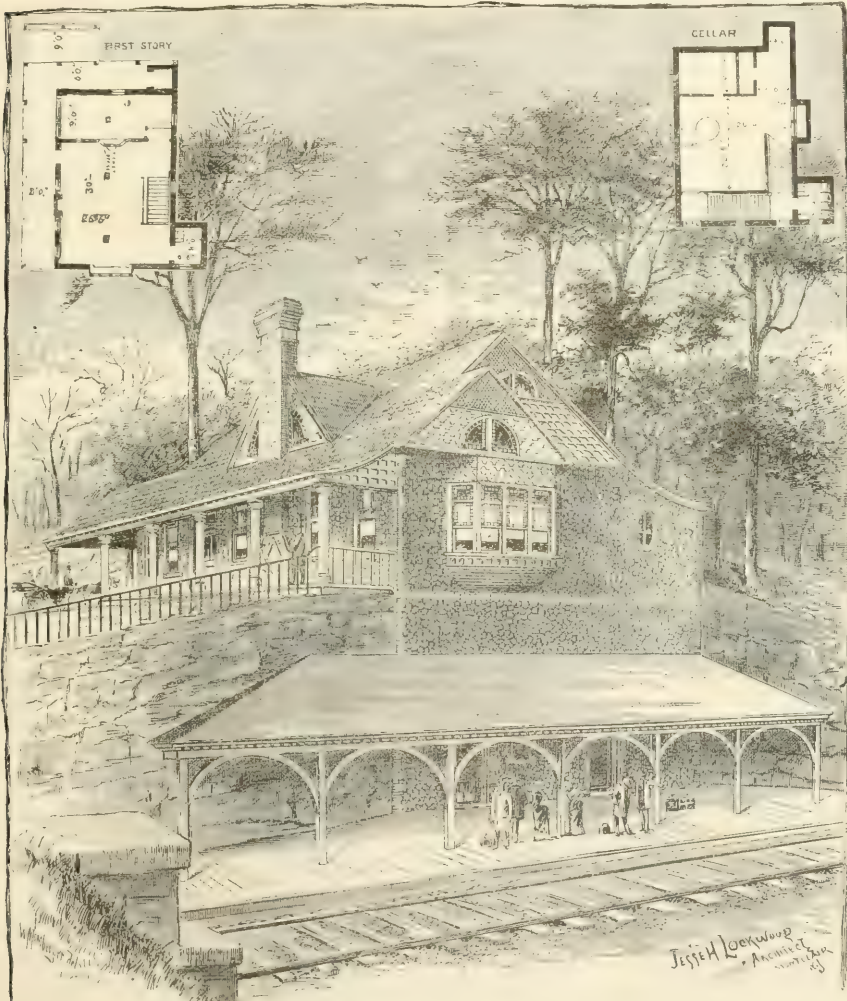
FIG. 587.—FIRST STORY PLAN.
