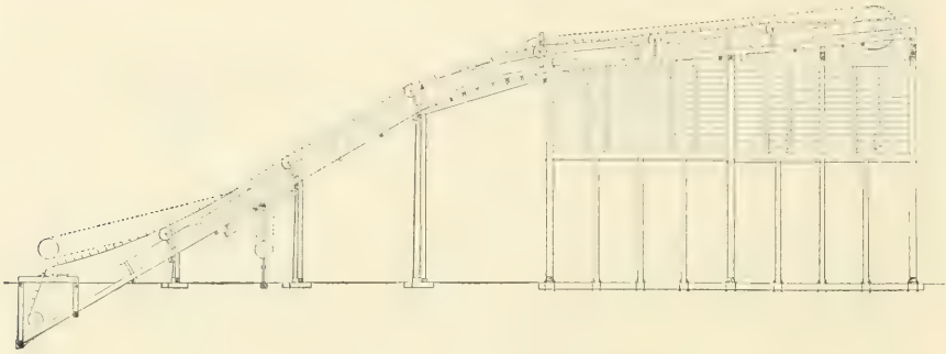
FIG. 287.—FRONT ELEVATION.
