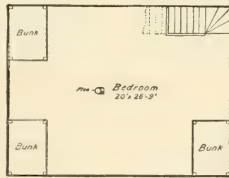
FIG. 60.—SECOND-FLOOR PLAN.
