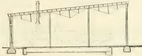
FIG. 341.—CROSS-SECTION.
