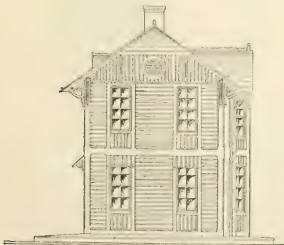
FIG. 510.—END ELEVATION.
