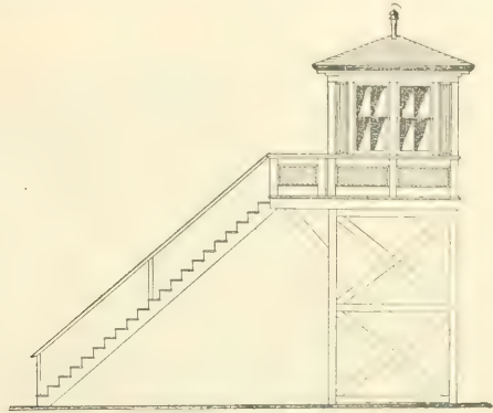
FIG. 120.—SIDE ELEVATION.
