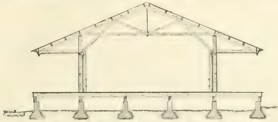
FIG. 463.—CROSS SECTION.
