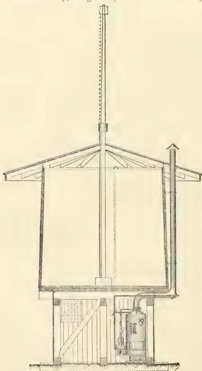
FIG. 159.—CROSS-SECTION.
