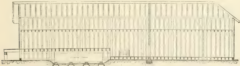
FIG. 199.—LONGITUDINAL SECTION.
