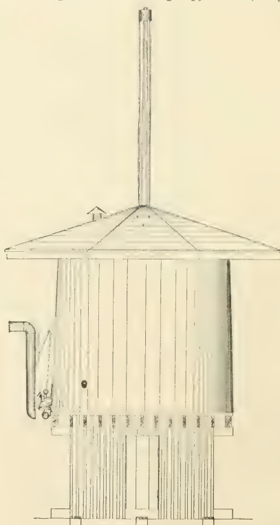
FIG. 260.—ELEVATION.
