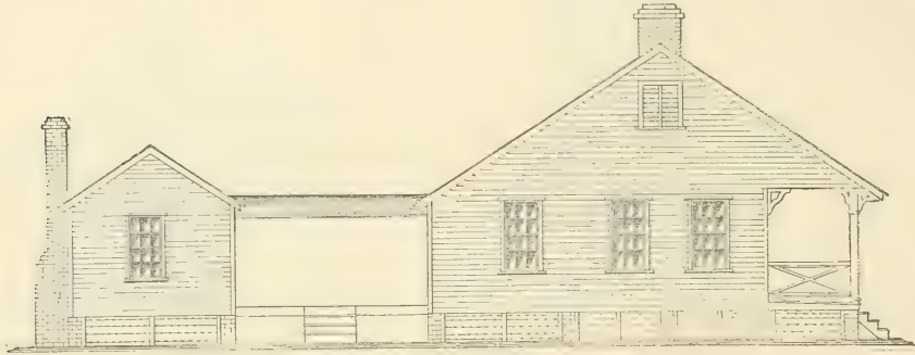
FIG. 61.—SIDE ELEVATION.
