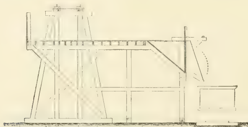
FIG. 279.—CROSS-SECTION.
