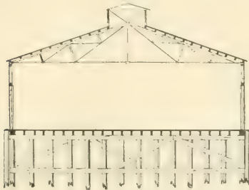
FIG. 396.—CROSS-SECTION.
