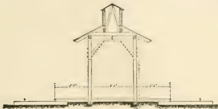
FIG. 139.—CROSS-SECTION.
