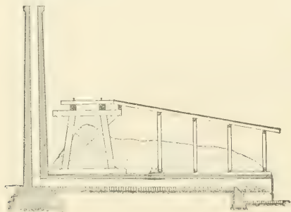
FIG. 183.—CROSS-SECTION.
