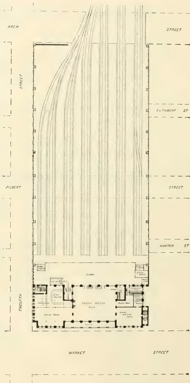
FIG. 686.—GROUND-PLAN OF TRAIN FLOOR.
