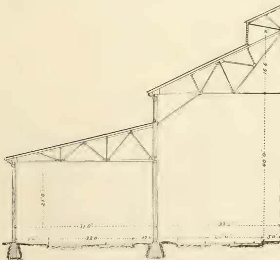
FIG. 657. CROSS-SECTION.
