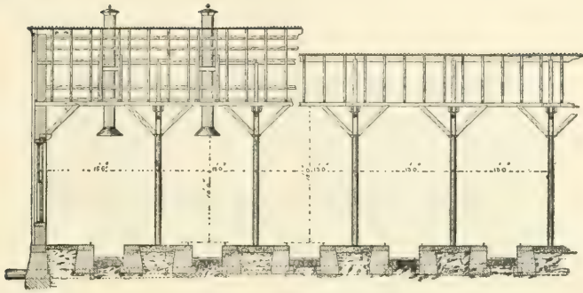
FIG. 344.—CROSS-SECTION.
