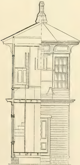
FIG. 115.—CROSS-SECTION AND FRONT ELEVATION.
