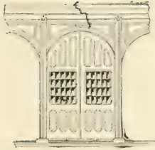
FIG. 318.—ELEVATION OF INTERIOR WALL AND ENGINE-DOOR.
