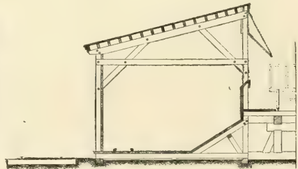
FIG. 270.—CROSS-SECTION.
