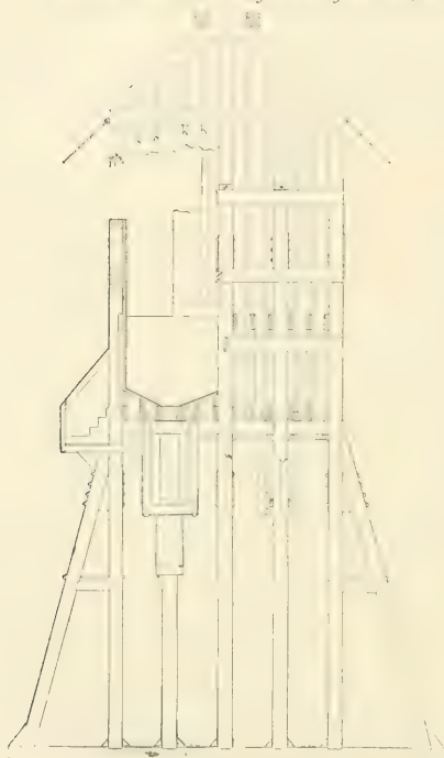
FIG. 290.—CROSS-SECTION.
