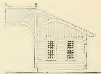
FIG. 419.—END ELEVATION.
