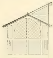
FIG. 30.—SIDE ELEVATION "A".
