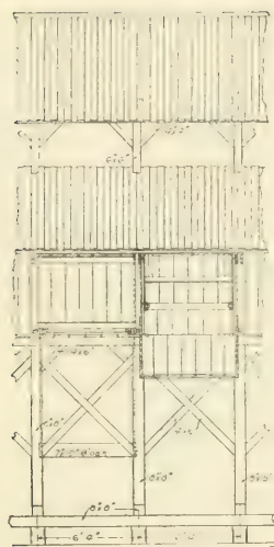
FIG. 291.—FRONT ELEVATION.
