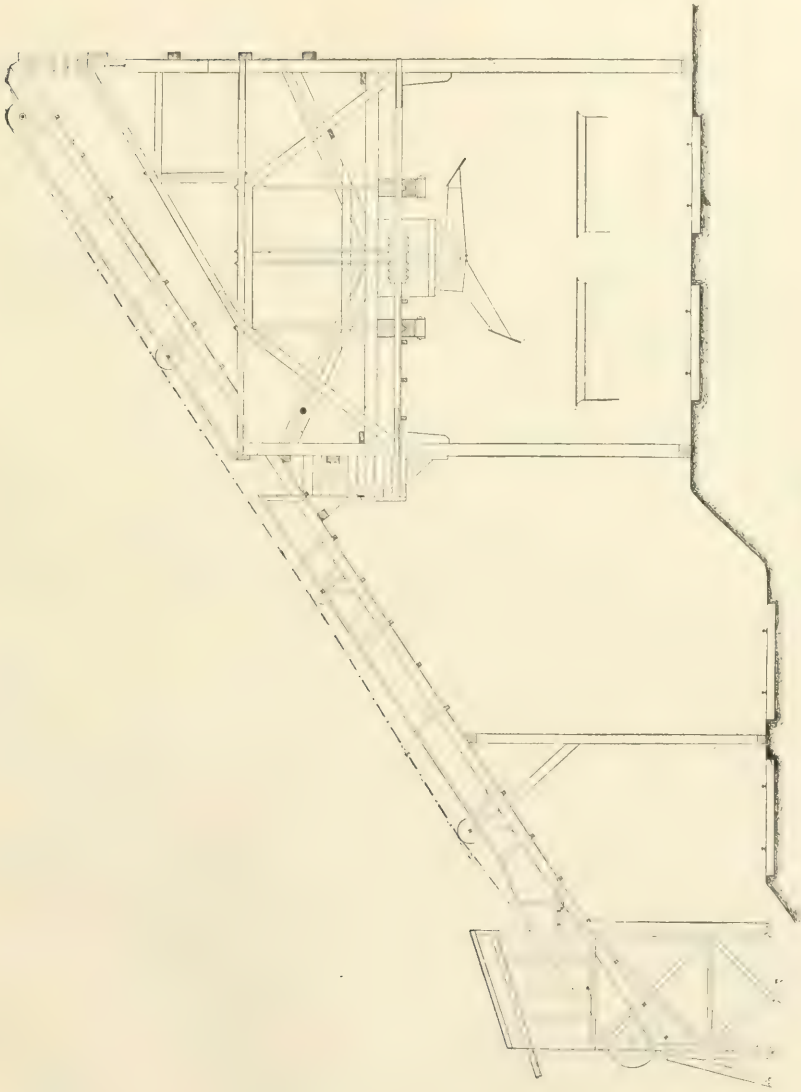
FIG. 289.—ELEVATION.
