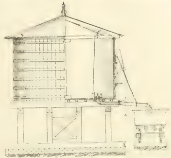
FIG. 246.—ELEVATION AND CROSS-SECTION.
