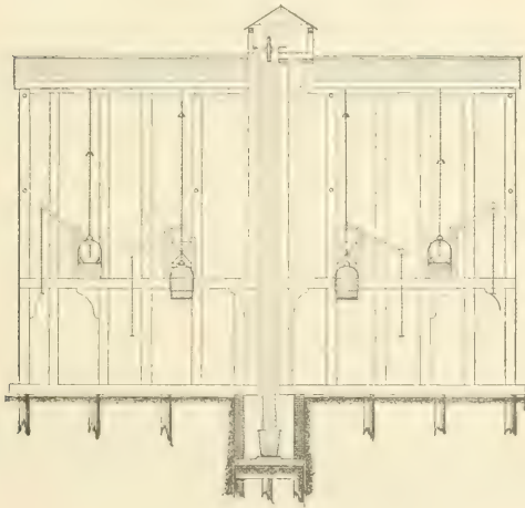
FIG. 285.—FRONT ELEVATION.
