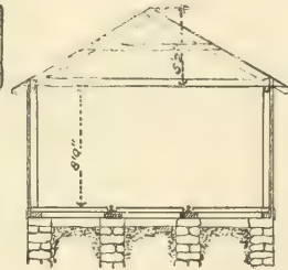
FIG. 20.—SECTION.
