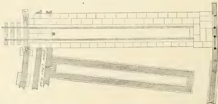
FIG. 317. GROUND PLAN.
