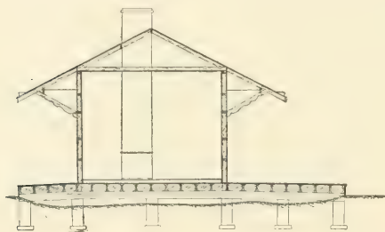
FIG. 443.—CROSS-SECTION.
