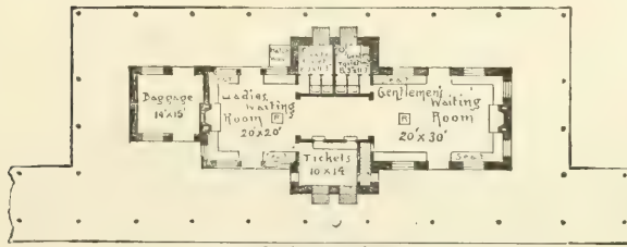
FIG. 603.—GROUND-PLAN, CHELTON AVENUE DEPOT.
