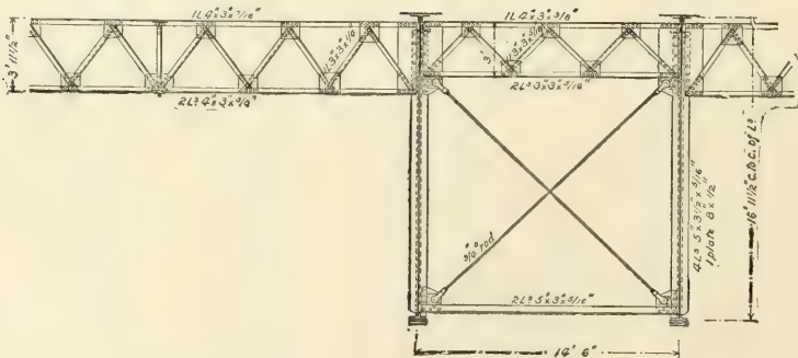
FIG. 661.—SECTION OF PAIR OF TRUSSES, SHOWING PURLINS.
