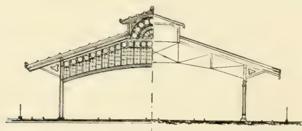
FIG. 643.—CROSS-SECTION AND END ELEVATION OF TRAIN-SHED.
