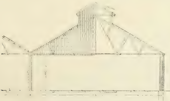
FIG. 630 — CROSS SECTION OF TRAIN-SHED.
