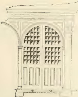
FIG. 306.—ELEVATION OF ENGINE-DOOR.
