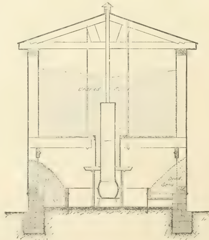
FIG. 180.—CROSS-SECTION.
