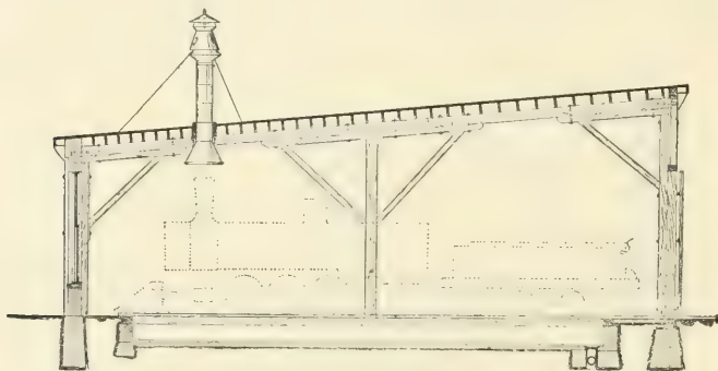
FIG. 339.—CROSS SECTION.
