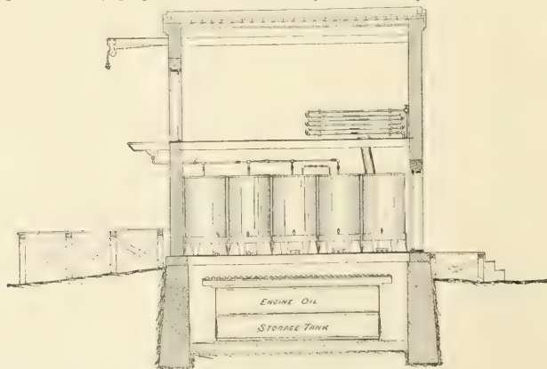
FIG. 210.—LONGITUDINAL SECTION.
