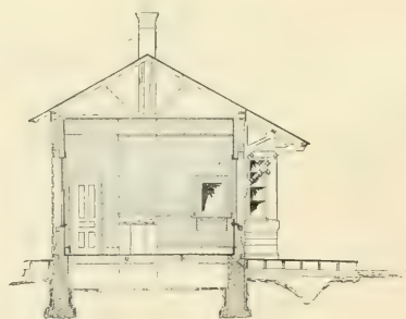
FIG. 556.—CROSS-SECTION.
