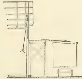
FIG. 162. — LONGITUDINAL SECTION.
