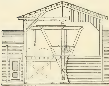
FIG. 269.—FRONT ELEVATION.
