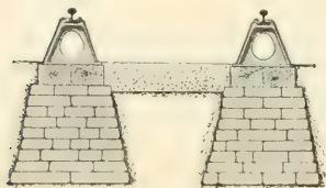
FIG. 150.—CROSS-SECTION.
