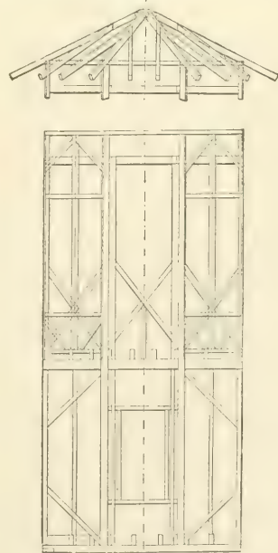
FIG. 116.—ELEVATION OF FRAME.
