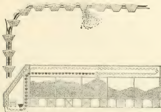
FIG. 302.—CROSS-SECTION OF HUNT CONVEYOR SYSTEM.
