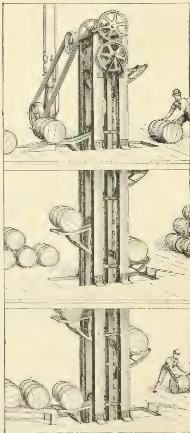
FIG. 392.—RUDDELL BARREL AND FREIGHT ELEVATOR.
