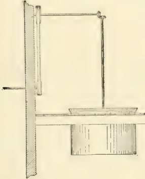
FIG. 219.—CROSS-SECTION.
