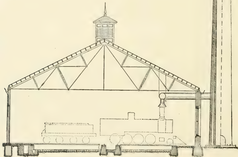
FIG. 316.—CROSS-SECTION.
