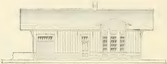
FIG. 452.—FRONT ELEVATION.
