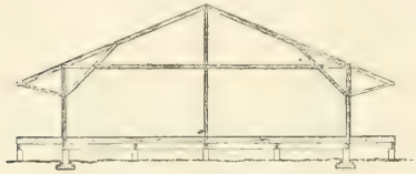
FIG. 373.—CROSS-SECTION
