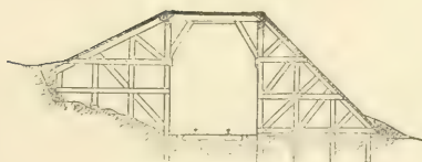
FIG. 109.—CROSS-SECTION.
