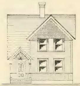
FIG. 83.—FRONT ELEVATION.
