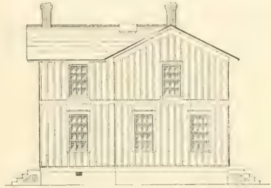
FIG. 85.—SIDE ELEVATION.
