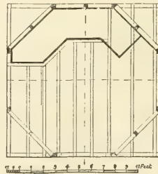
FIG. 118.—SECOND-FLOOR FRAMING PLAN.
