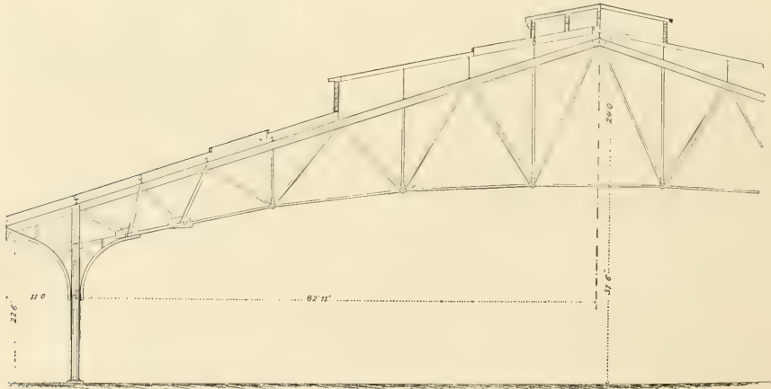
FIG. 675.—CROSS-SECTION OF TRAIN-SHED.
