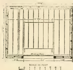
FIG. 28.—GROUND-PLAN "A" AND "B".
