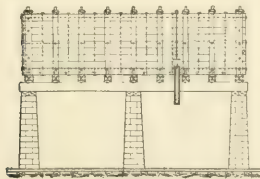
FIG. 247.—FRONT ELEVATION.
