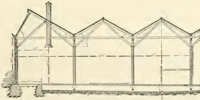
FIG. 345.—LONGITUDINAL SECTION.
