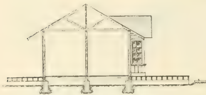
FIG. 469. - CROSS-SECTION.
