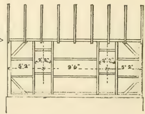
FIG. 21.—ELEVATION OF FRAME.
