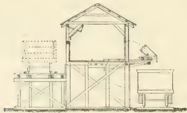
FIG. 277.—CROSS-SECTION.
