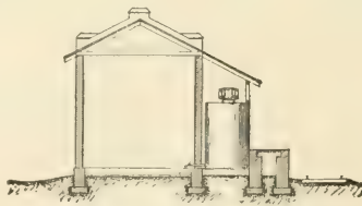
FIG. 196.—CROSS SECTION.
