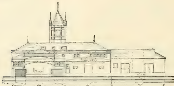
FIG. 399.—ELEVATION FROM RIVER.
