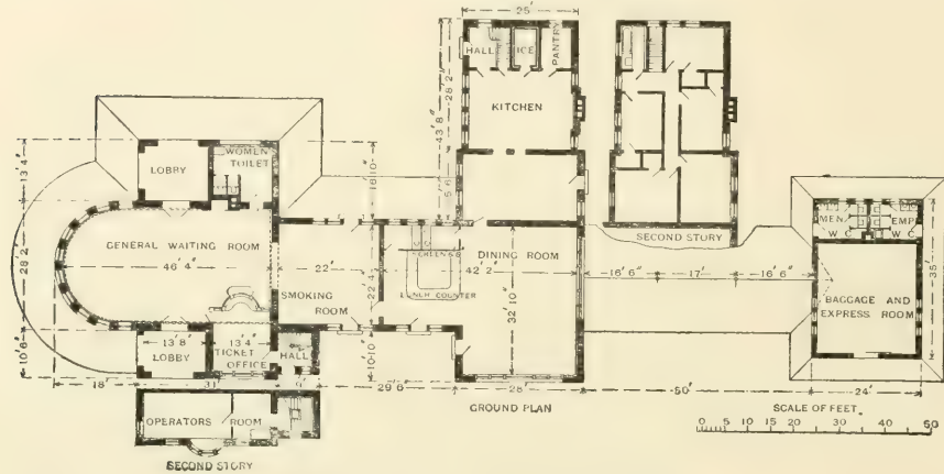
FIG. 620.—GROUND-PLAN AND SECOND-STORY PLAN.
