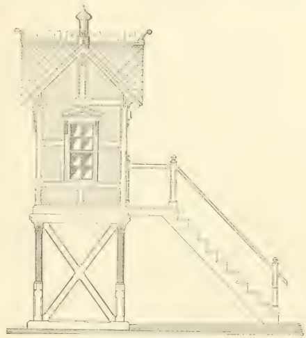
FIG. 114.—SIDE ELEVATION.
