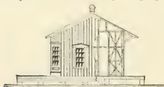
FIG. 474.—END ELEVATION AND CROSS-SECTION.
