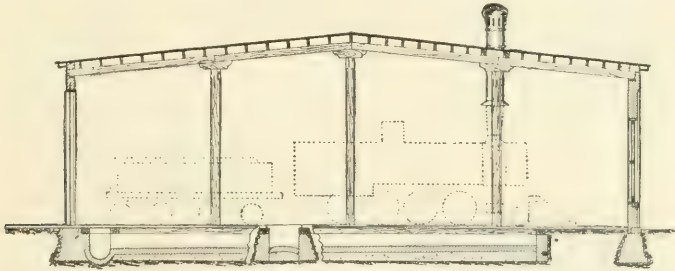
FIG. 329.—CROSS SECTION.
