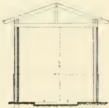
FIG. 132.—CROSS SECTION.
