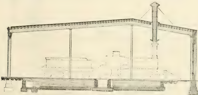
FIG. 323.—CROSS-SECTION.
