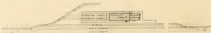
FIG. 422.—PROPOSED GENERAL LAYOUT FOR A COMBINATION DEPOT.
