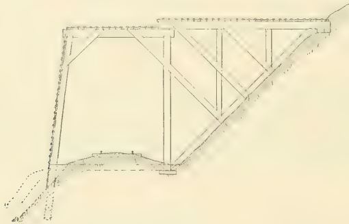
FIG. 106.—CROSS-SECTION.
