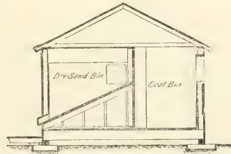
FIG. 177.—CROSS-SECTION.
