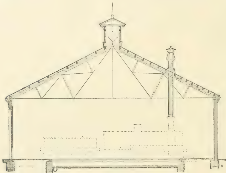
FIG. 308.—CROSS SECTION.
