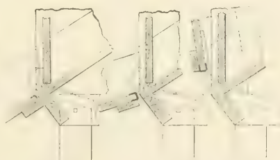
FIG. 294.—DETAIL OF POSITIONS OF APRON.
