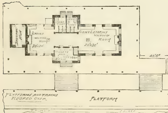
FIG. 604.—GROUND-PLAN, CHESTNUT HILL DEPOT.
