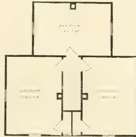
FIG. 87.—SECOND-FLOOR PLAN.
