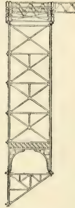
FIG. 660.—CROSS-SECTION OF WIND-BRACING AT END OF TRAIN-SHED.
