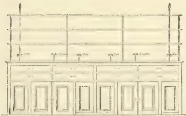
FIG. 237.—FRONT ELEVATION OF LABORATORY TABLE.
