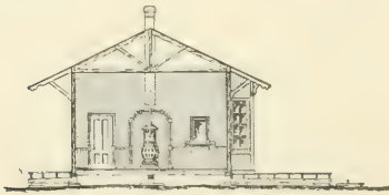
FIG. 427.—CROSS-SECTION, CLASS "E."
