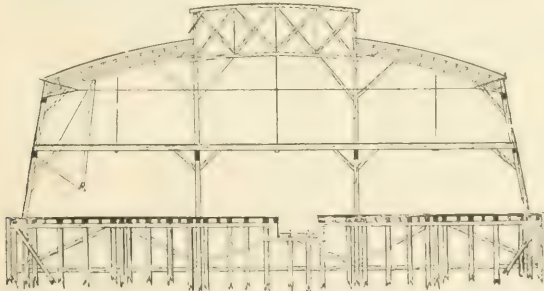
FIG. 394. CROSS SECTION
