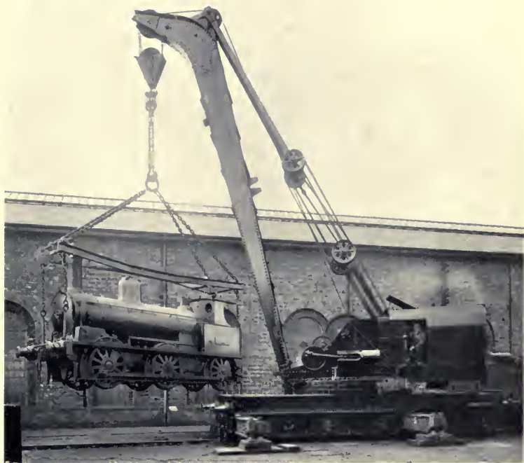
BREAKDOWN CRANE AND LIFTING TACKLE FOR SHIPPING SMALL GOODS ENGINES.
