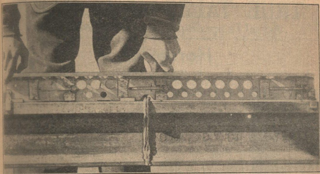
A Close-Up of the Alignment Gage. Original Thermite Welds Had a Tendency to Soften the Webs, Depressing the Rail Heads at the Joints
