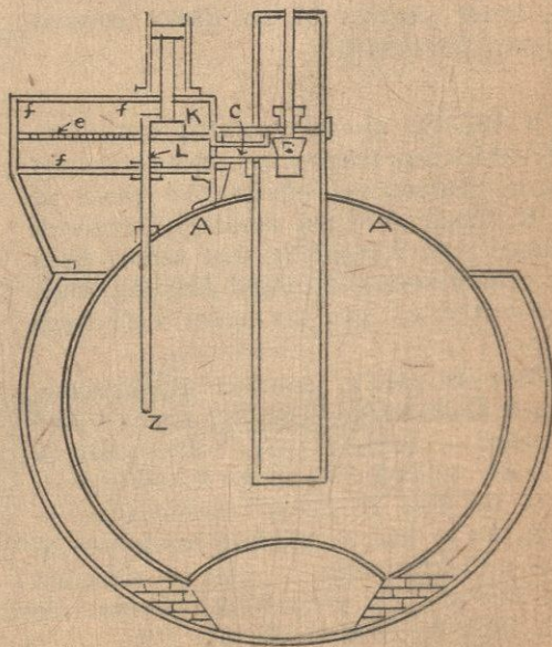
Trevithick's Feedwater Heater. Cylinder Exhaust Steam Was Admitted via Passage (c) to Water-Filled Cistern (f), Heating Supply as It Filtered through Perforations (e). Pump (k) then Jetted Water into Pipe (l) to Boiler (A) at z
