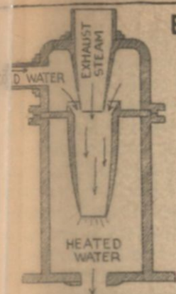
D.K. CLARK'S THREE PLANS FOR INJECTION OR OPEN TYPE HEATER. THE EXHAUST STEAM MIXES DIRECTLY WITH THE COLD FEEDWATER
