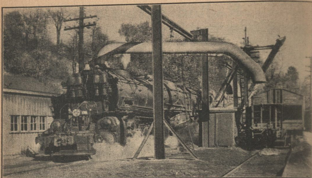
Photo by Kenneth H. Cooke, 3407 Clifton Ave., Cincinnati, Ohio To Keep Dust from the Nearby "Spotless" Town of Mariemont, O., Suburb of Cincinnati, the Norfolk & Western Puts Pipes Over Locomotive Stacks in the Clare Yards. Running Water Wets Down the Ashes, Diverts Them into a Car
