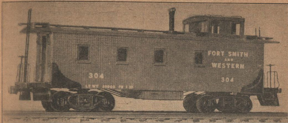
Preston George, of 2235 Newton St., Denver, Colo., Built This Excellently Detailed O-Gauge Caboose with No Commercial Parts Other than Trucks. Faithful to Prototype, Its Body Is Fashioned of Wood—in This Case, the Sides of a 5-Pound Cheese Box. Steps of Soldered Tin Can Stock Incorporate a Crispness of Detail Not Found in Castings.
