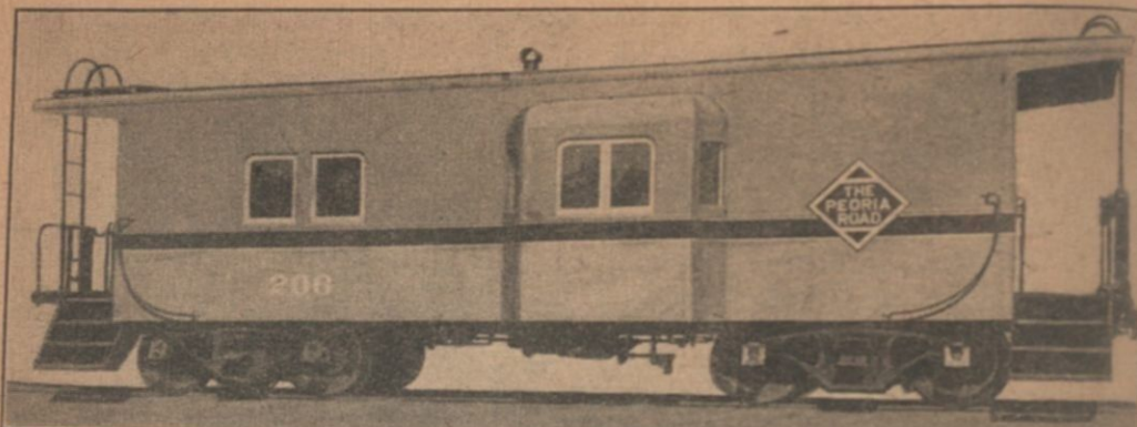
Semi-Streamlined Steel Caboose of the Toledo, Peoria & Western: Half a Dozen Were Designed and Built Recently at the Company's East Peoria Shops
